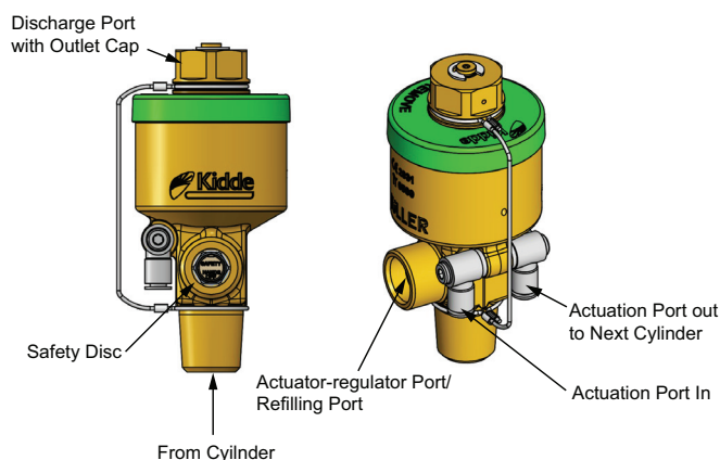
Figure 3. Valve Components
