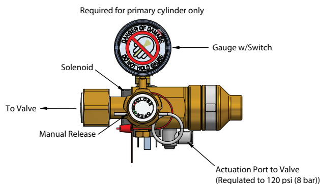
Figure 4. Release Unit
