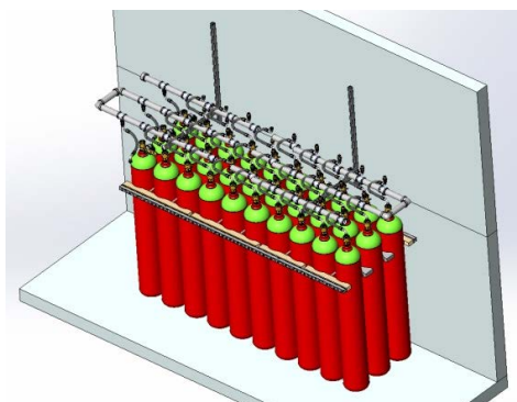
Figure 15. 80L Cylinder Racking Example
