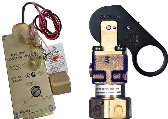
Electric Control Head
