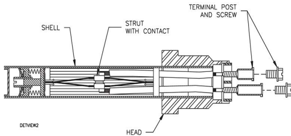
Figure 2. Detector Internal View
