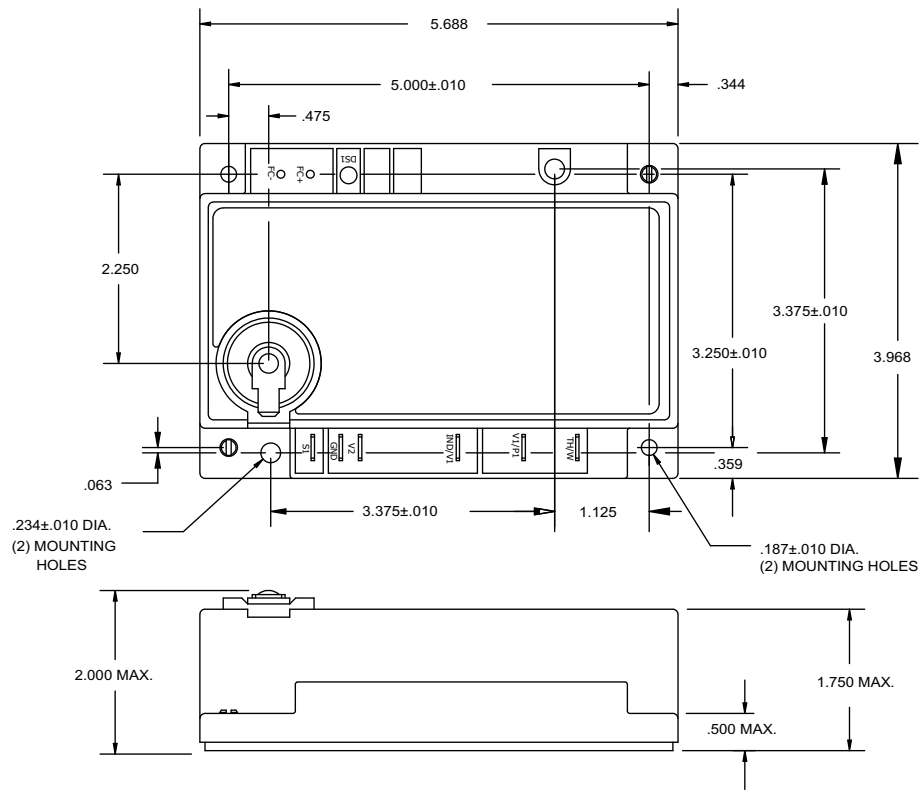
Figure 5. Standard Enclosure
