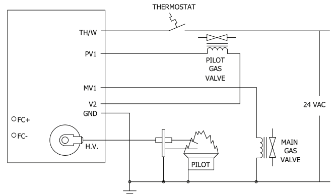
Figure 1. Local Sense
