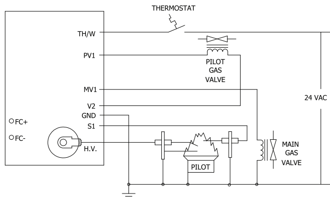
Figure 2. Remote Sense
