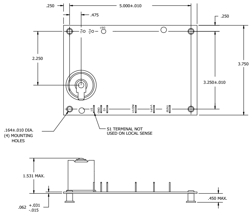
Figure 4. Uncovered with Standoffs
