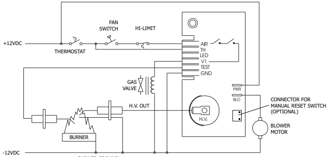
Figure 3. Remote sense with blower relay
