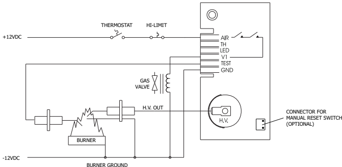
Figure 1. Remote sense without blower relay
