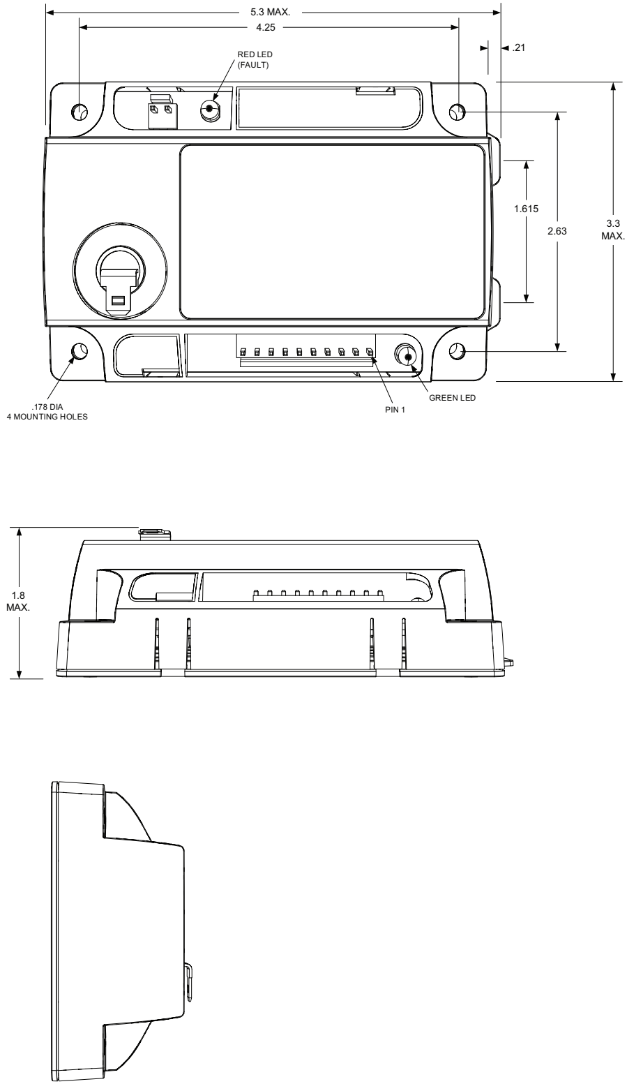
Figure 3. Standard Enclosure
