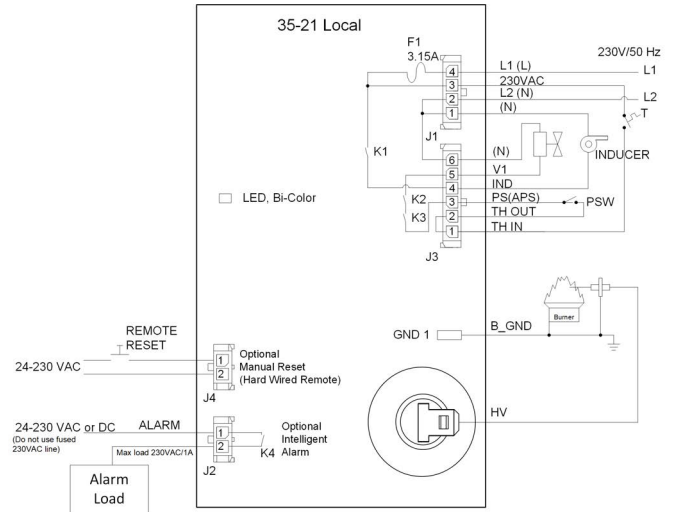
Figure 1. Local Sense
