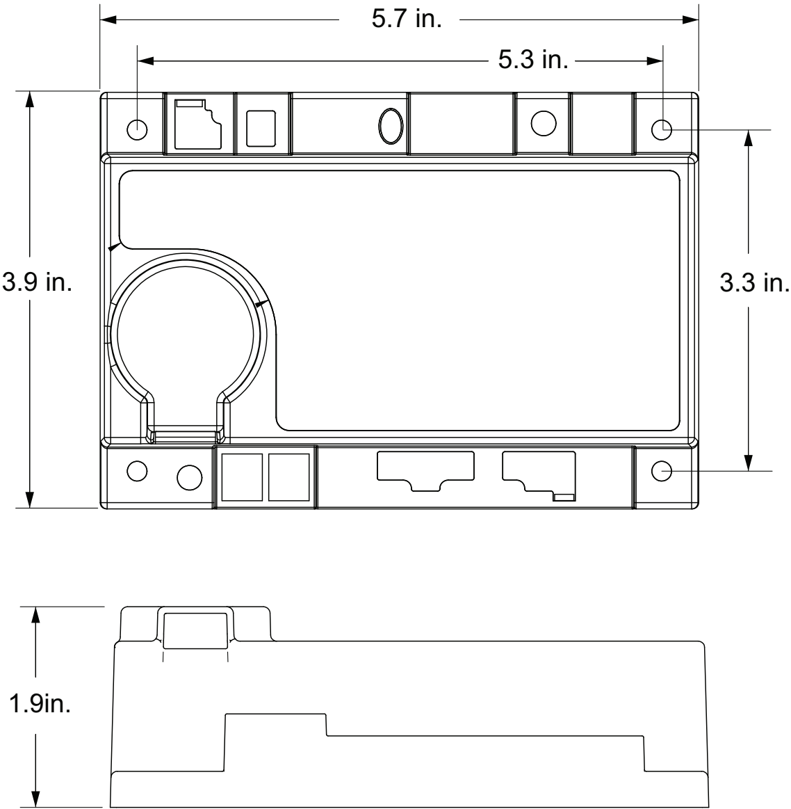
Figure 3. Standard Enclosure
